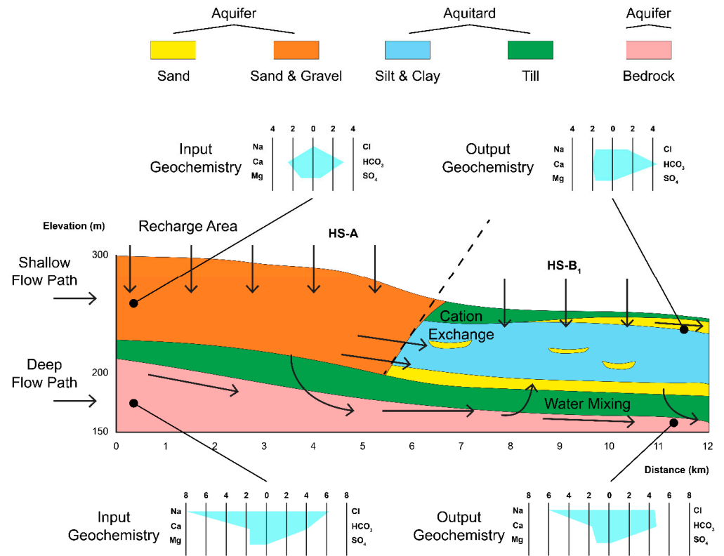
Figure 9. Conceptual model for the southern flow path.
