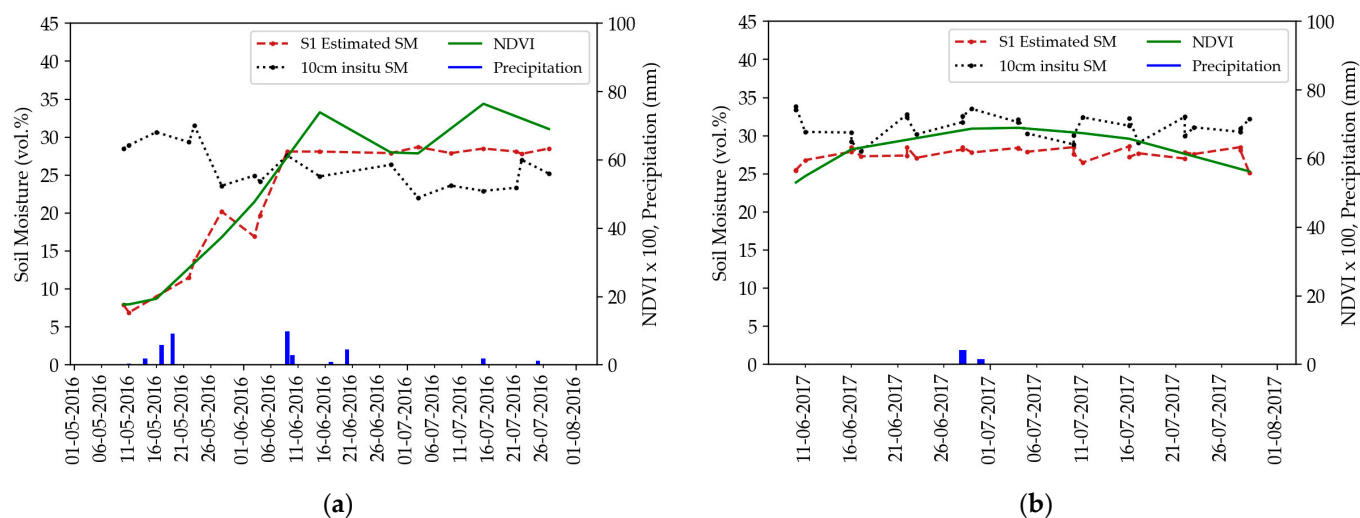
Figure 6. Temporal variation in the in situ 10 cm measured SM (black dotted line) and the S1 estimated SM (red dashed line) for (a) tomato crop cycle in IT-LAZ 2016 and (b) tomato crop cycle in IT-LAZ 2017. The NDVI is represented by a solid green line on the right y-axis, along with precipitation (blue line).
