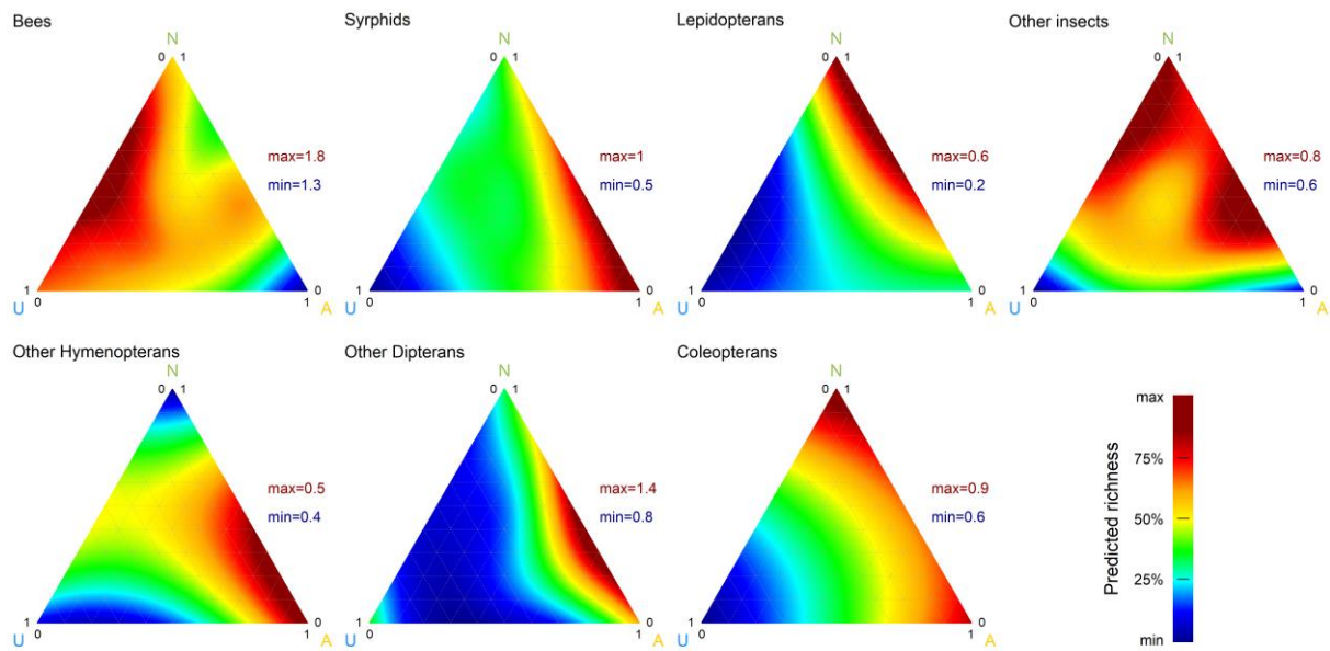
549 Fig. 8. Ternary diagram of the percentage accessibility to urban (U), agricultural (A) and semi-natural 550 (N) land-cover classes showing the predicted landscape effect on the richness of each insect taxa. The 551 min and max represent the minimum and maximum predicted values, respectively.
