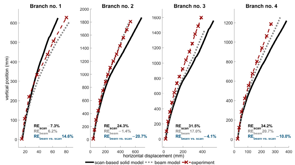
Figure 7. Experimental validation of beam and scan-based solid FEMs for horizontal loading. Relative error (RE) refers to the relative error of the sum of horizontal displacements. The presented relative errors are for comparison of beam ( RE_{\text{beam}} ) and scan ( RE_{\text{scan}} ) with experiment, and also for comparison of beam and scan-based solid geometry ( RE_{\text{beam vs. scan}} ).
