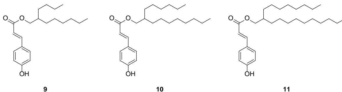
Figure 1. Structure of 2-butyl octyl p -hydroxycoumarate 9 ; 2-hexyl decyl p -hydroxycoumarate 10 ; and 2-octyl dodecyl p -hydroxycoumarate 11 .
