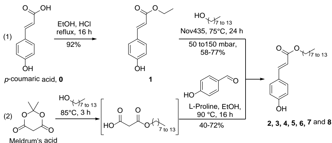
Scheme 1. Synthesis of the alkyl p -hydroxycoumarates through a chemo-enzymatic pathway (1) or green Knoevenagel-Doebner condensation (2).
