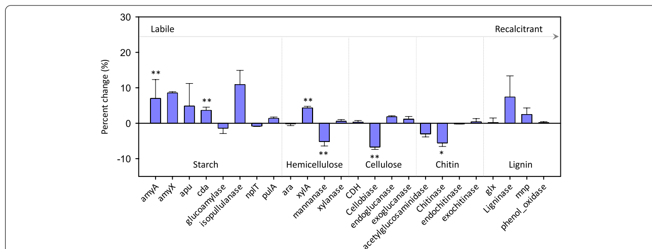
Fig. 2 Changes in C cycling gene abundances. The percent change in the relative abundance of C degradation genes by N deposition is calculated as 100*((mean value in N deposited samples/mean value in control samples) - 1). Mean values and standard deviations are presented. Asterisks indicate significant differences. * P < 0.050 ; ** P < 0.010
