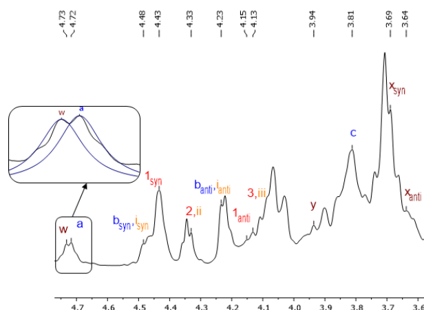
Figure 2. Typical ^1\text{H} NMR ( \text{DMSO}-d_6 ) spectrum of the PC structure (#7, Table 1) shown in Scheme 3 (see SI for the full ^1\text{H} -NMR spectrum)
