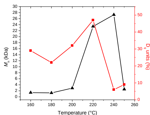
Figure 4. Effect of polycondensation temperature on M_n and polymer branching
