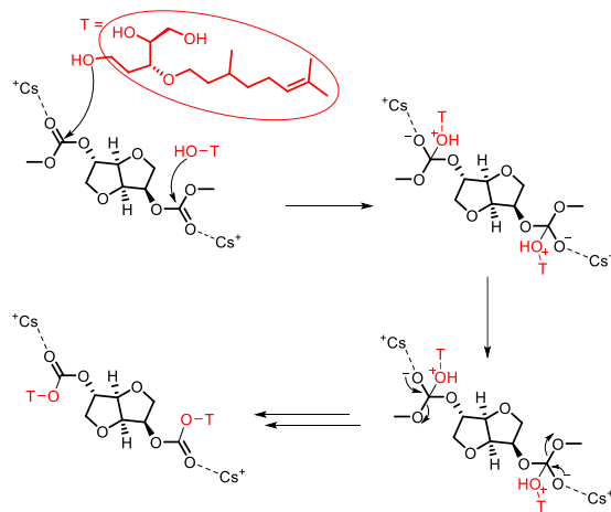
Scheme 4. Polycondensation mechanism of Triol-Citro and DCI catalysed by \text{Cs}_2\text{CO}_3
