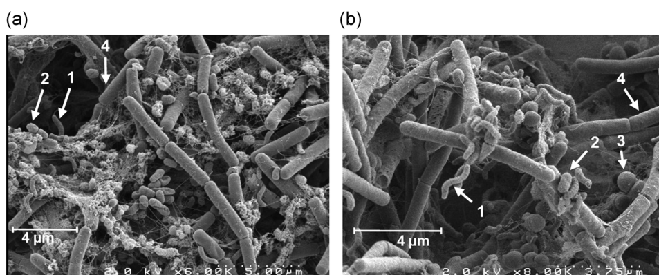
FIGURE 2 Physical Interactions between species in the biofilm. Scanning electron micrograph of the four-species biofilm at T = 72 h (a) and of a biofilm grown under identical conditions but containing a Bacillus cereus \Delta tclE-H mutant lacking thiocillin production in place of the wild-type strain (b). The four species are indicated by arrows in panels a and b: (1) Rhodocyclus , (2) Pseudomonas fluorescens , (3) Kocuria varians , (4) B. cereus . Note that in biofilms containing the wild-type B. cereus , K. varians numbers are much reduced, such that none are observed in the image (a) which is representative of the majority of the observed microscopic fields. Scales are shown at the bottom right
