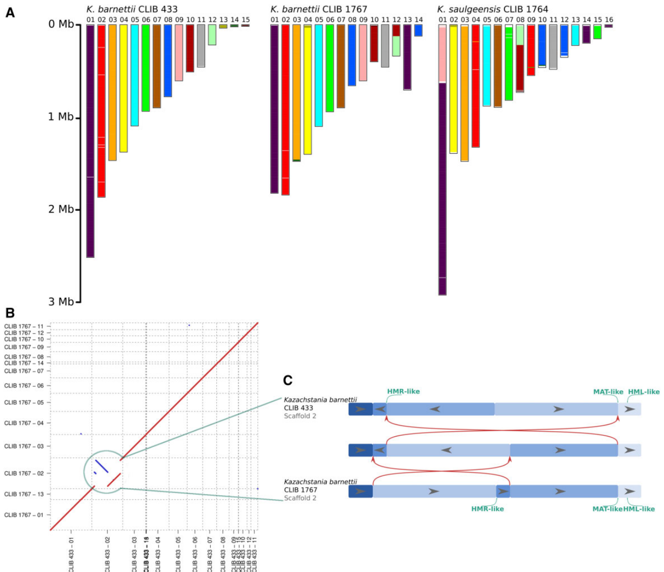
FIG. 1. —(A) Synteny blocks between the Kazachstania barnettii strains CLIB 433 (reference) and CLIB 1767 (sourdough) and the Kazachstania saulgeensis strain CLIB 1764 (sourdough) Each synteny block is colored according to the scaffolds of CLIB 433. Thus, for example, blocks from the scaffold 01 in CLIB 433 (in violet) are found in scaffolds 01 and 13 in the assembly of CLIB 1767 and in scaffolds 01, 14, and 16 in the assembly of K. saulgeensis CLIB 1764. (B) Dot plot between the two K. barnettii strains, CLIB 433 (reference) and CLIB 1767 (sourdough) based on MUMmer matches. To facilitate reading and interpretation of, scaffolds are reordered in accordance with the synteny block organization in (A). (C) Comparison of the structure of the scaffolds of the two K. barnettii assemblies. Red arrows represent possible inversion events between the two scaffolds in one possible sequence leading from one strain’s organization to the other. The central band represents the corresponding intermediate organization. Positions of mating type loci are indicated in green.
