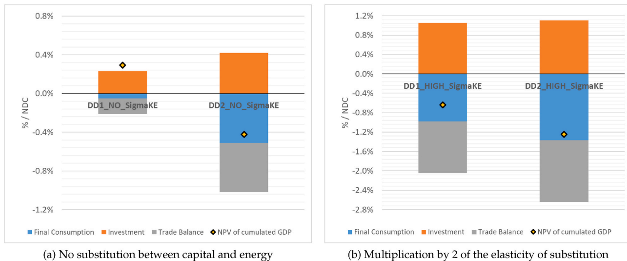
Fig. 9. Sensitivity analysis for substitution between capital and energy in non-energy sectors - NPV of cumulated GDP losses (2015–2050) in DD scenarios compared to NDC discounted at a 5% discount rate and mean annual incremental difference of GDP components as shares of GDP compared to NDC.
