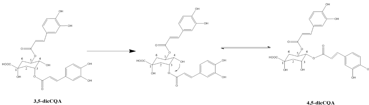
Figure 6. Isomerization reaction of 3,5-O-di-CQA to 4,5-O-di-CQA.
