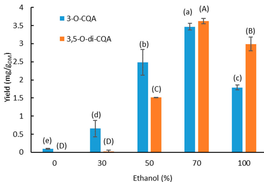
Figure 2. Effect of the percentage of ethanol in the extraction solvent on the extraction yield of 3-O-CQA and 3,5-O-di-CQA at ( T = 30\text{ }^{\circ}\text{C} ; S/L = 1/50 ; t = 24\text{ h} ). Bars with different small letters indicate significant differences in the yield of 3-O-CQA ( p > 0.05 ) according to the Tukey test at 95%. Bars with different capital letters indicate significant differences in the yield of 3,5-O-di-CQA.
