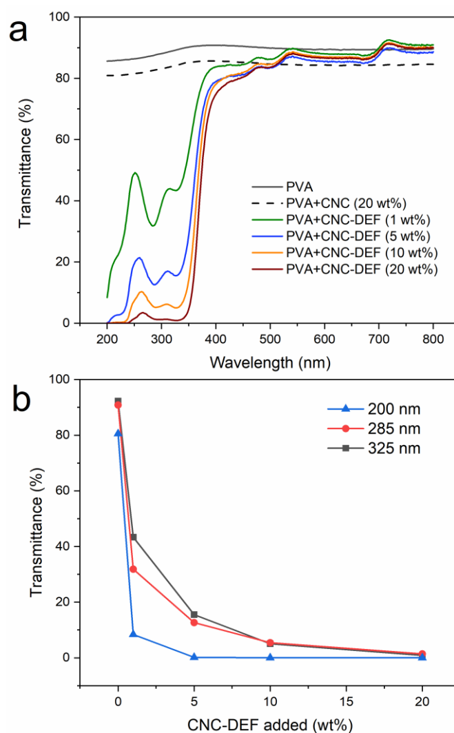
Figure 5. UV-blocking property of PVA+CNC-DEF composite films. (a) UV-Vis transmittance spectra of neat PVA, PVA+CNC (20 wt%), and PVA+CNC-DEF (1-20 wt%) composite films. (b) Optical transmittance of PVA+CNC-DEF films at different UV wavelengths.
