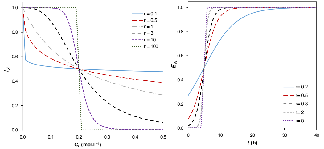
Figure 3. (a) Example of inhibition factor I_X as a function of C_I for different n values and K_{IX} = 0.2 mol L -1 . (b) Example of enzymatic activation factor E_A as a function of t for different r values, and t_{lag} = 5 h.
