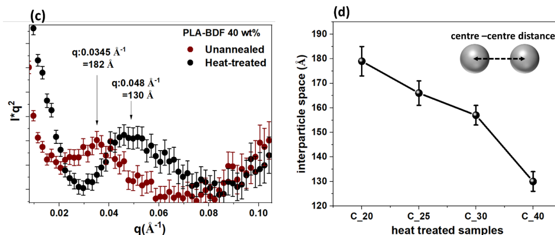
Figure 6: Small angle X-ray Scattering (SAXS) curves of: (a) unannealed PLA and PLA blended with different dosage of BDF ranging from 0-40 wt%. Inset showed the Kratky plot of the SAXS curves. (b) SAXS of the heat-treated PLA and PLA blended with different BDF concentrations. The samples were heat-treated at 50 °C for 24 h. Inset showed the Kratky plot of the SAXS curves. (c) Kratky plot of the SAXS curves of the unannealed and heat-treated PLA-BDF 40 wt% samples; (d) Interparticle distance of heat-treated PLA blended with BDF 20, 25, 30 and 40 wt%.
