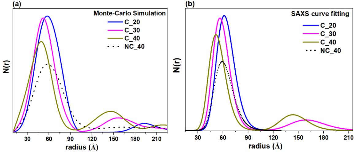
Figure 7: Size distribution from unannealed PLA with 40 wt% BDF and heat-treated PLA blended with different BDF concentrations (20 - 40 wt%). (a) Size distribution calculated by Monte Carlo simulation; (b) Size distribution obtained from SAXS curve fitting.
