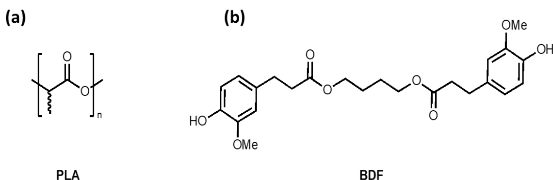
Figure 1: (a) Monomer unit of lactic acid. (b) Monomer unit of Bis- O -feruloyl-1,4-butanediol (BDF)
