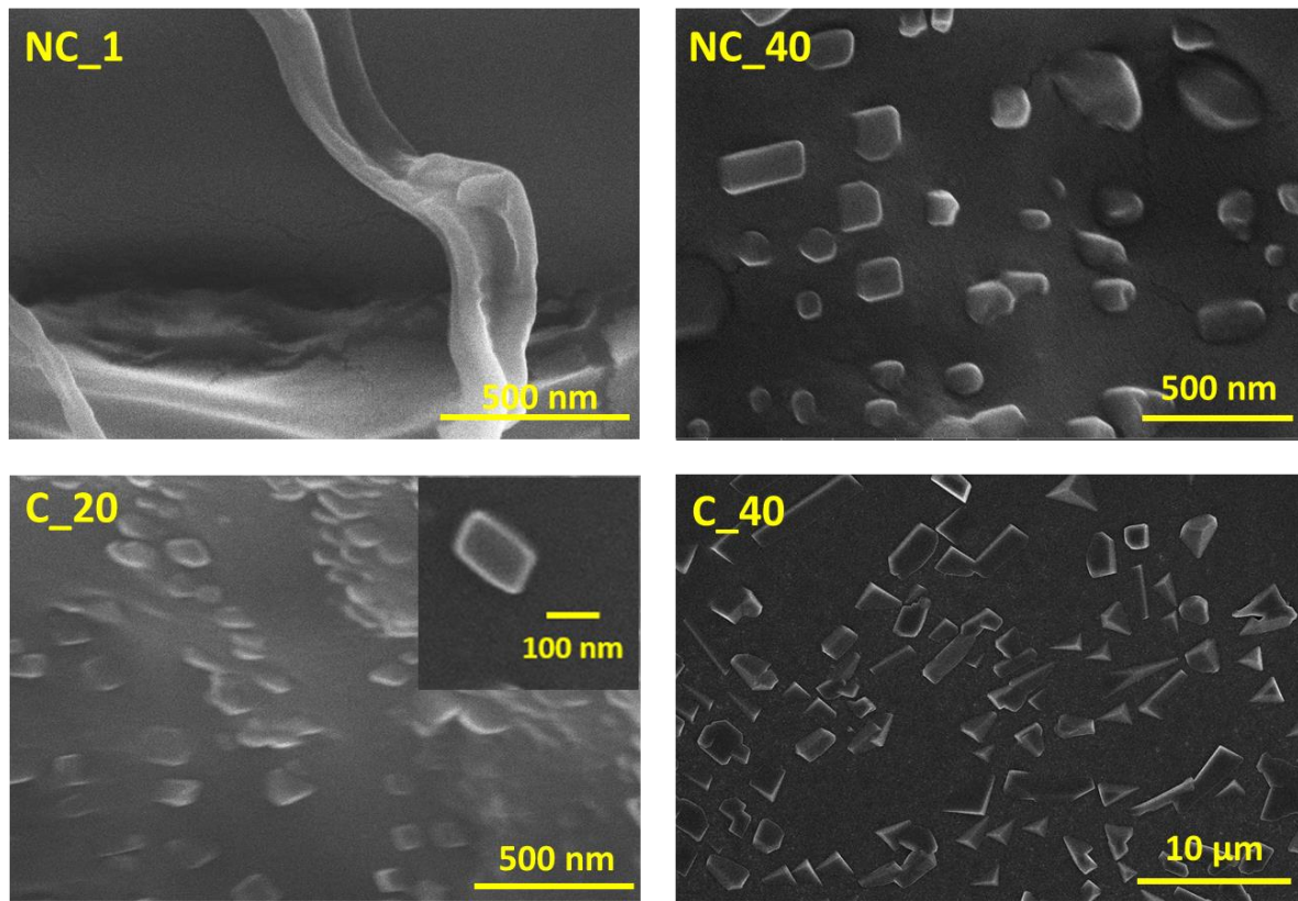
Figure 4: Scanning electron micrographs (SEM) of the unannealed PLA (NC_1) and PLA-BDF 40 wt% (NC_40). The bottom row shows the SEM of heat-treated PLA-BDF 20 wt% (C_20) and PLA-BDF 40 wt% (C_40). The samples were heat treated at 50 °C for 24 h.
