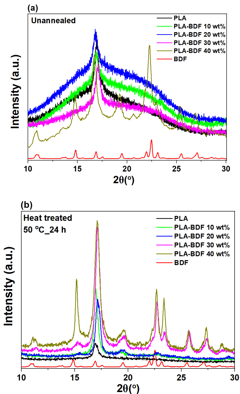
Figure 5: X-ray diffraction (XRD) of (a) unannealed PLA and PLA blended with different BDF concentration varying from 10-40 wt%. (b) XRD of the heat-treated PLA and PLA-BDF blends with different BDF concentrations. The samples were heat-treated at 50 °C for 24 h.
