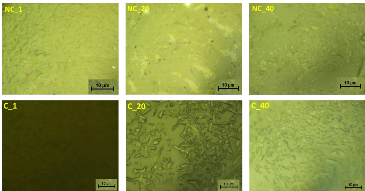
Figure 3: Polarised optical microscope (POM) images of the unannealed PLA (NC_1), PLA-BDF 20 wt% (NC_20) and PLA-BDF 40 wt% (NC_40). The bottom row shows the POM images of the heat-treated (annealed) homologous series: pure PLA (C_1) and PLA-BDF 20 wt% (C_20) and PLA-BDF 40 wt% (C_40). The samples were heat treated at 50 °C for 24 h. The scale bar represents 10 µm.
