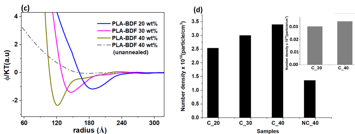
Figure 8: (a) Structure factor, (b) Radial distance distribution, (c) Potential mean force and (d) number density all extracted from the SAXS curves fitting for the unannealed PLA with 40 wt% BDF and heat-treated PLA blended with different BDF concentrations (20 -40 wt%).
