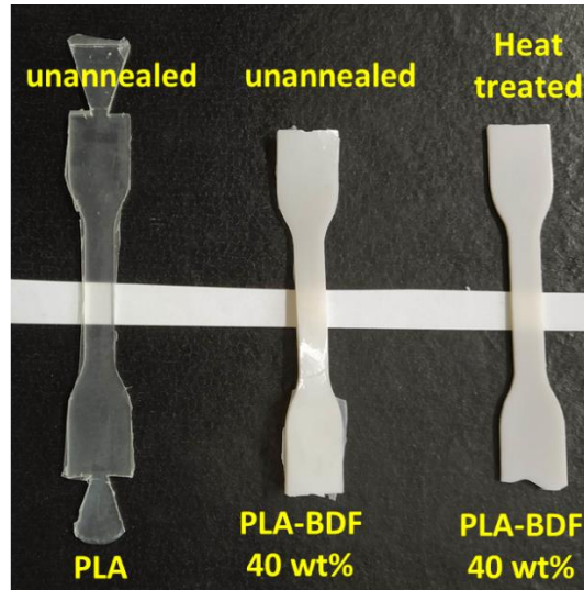
Figure 2: Images of the original (unannealed) transparent PLA (left); PLA blended with 40 wt% BDF (mid); and heat-treated PLA-BDF 40 wt% blend at 50 °C for 24 h (right).
