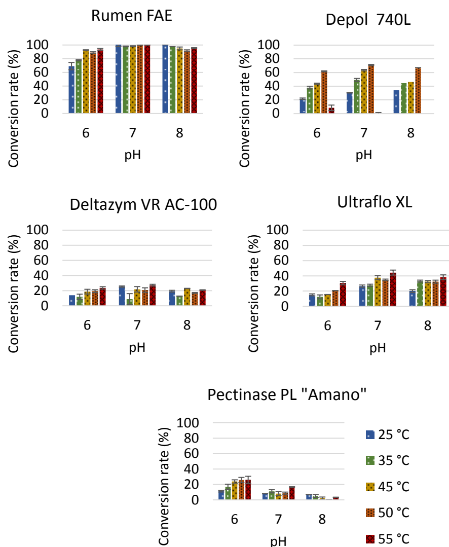
Figure 2: Conversion rate of sinapine chloride into sinapic acid with enzymatic solutions for 10 min with n = 2 .
