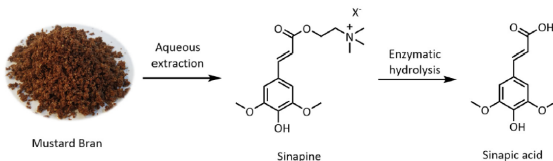
Figure 1: Enzymatic hydrolysis of mustard bran for the recovery of sinapic acid.
