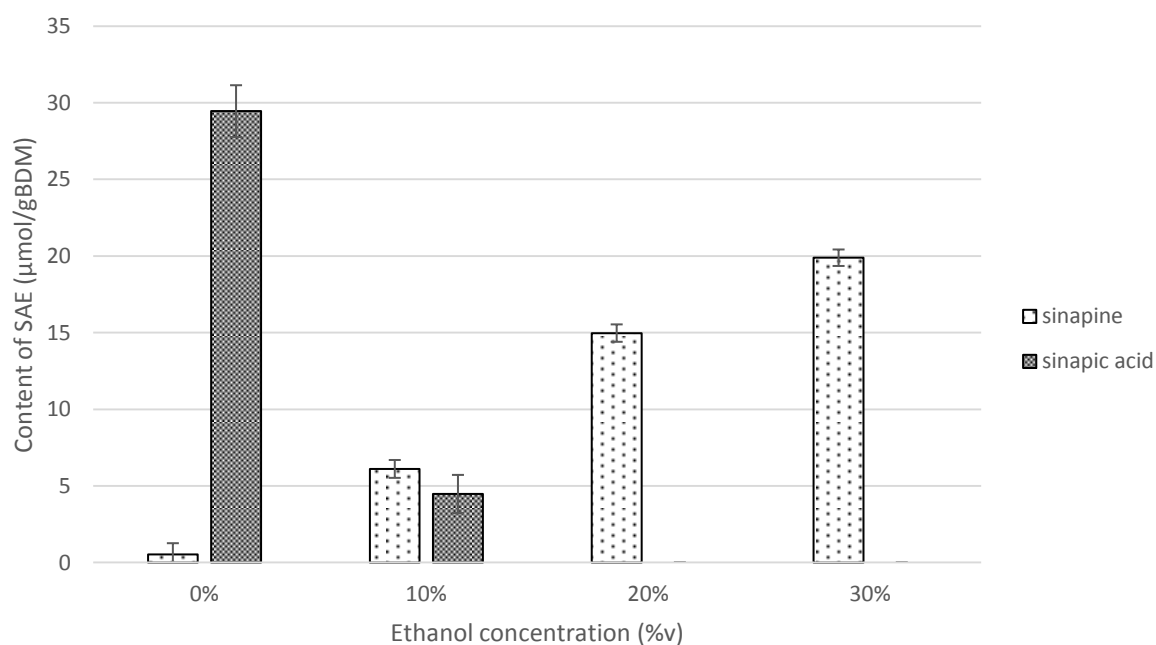
Fig. S2. Sinapic acid equivalent content for the simultaneous extraction and hydrolysis with rumen FAE under different ethanol concentration at 50 °C, pH 7 with n = 2
