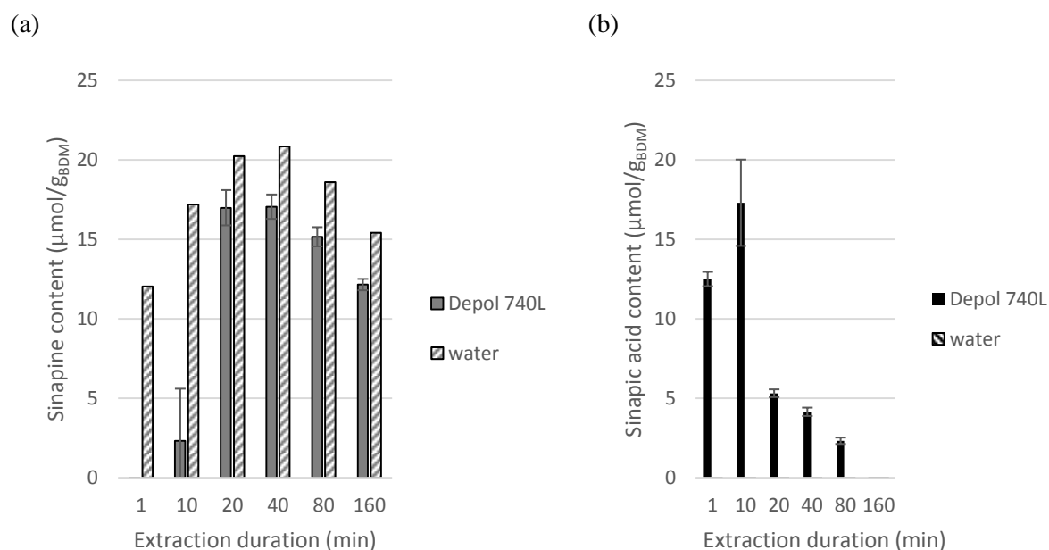
Fig. S1. Monitoring of hydrolysis kinetics during extraction of sinapic acid equivalents from mustard bran with Depol 740L and without enzymes at 75 °C, pH 7, n = 2.
