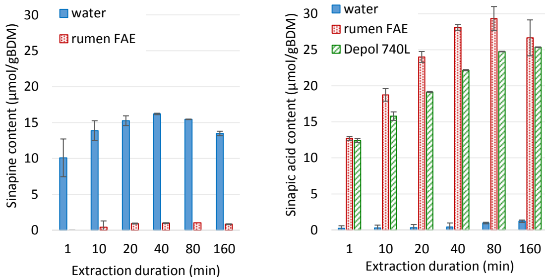
Figure 5: Sinapine content (a) and sinapic acid content (b) obtained from mustard bran with Depol 740L, rumen FAE and water at 50 °C, pH 7 during 160 min with n = 2 .
