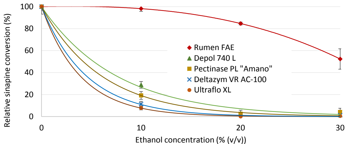
Figure 3: Sinapine chloride conversion rate with enzymatic solutions in function of ethanol concentration for 30 min ( n = 3 ).
