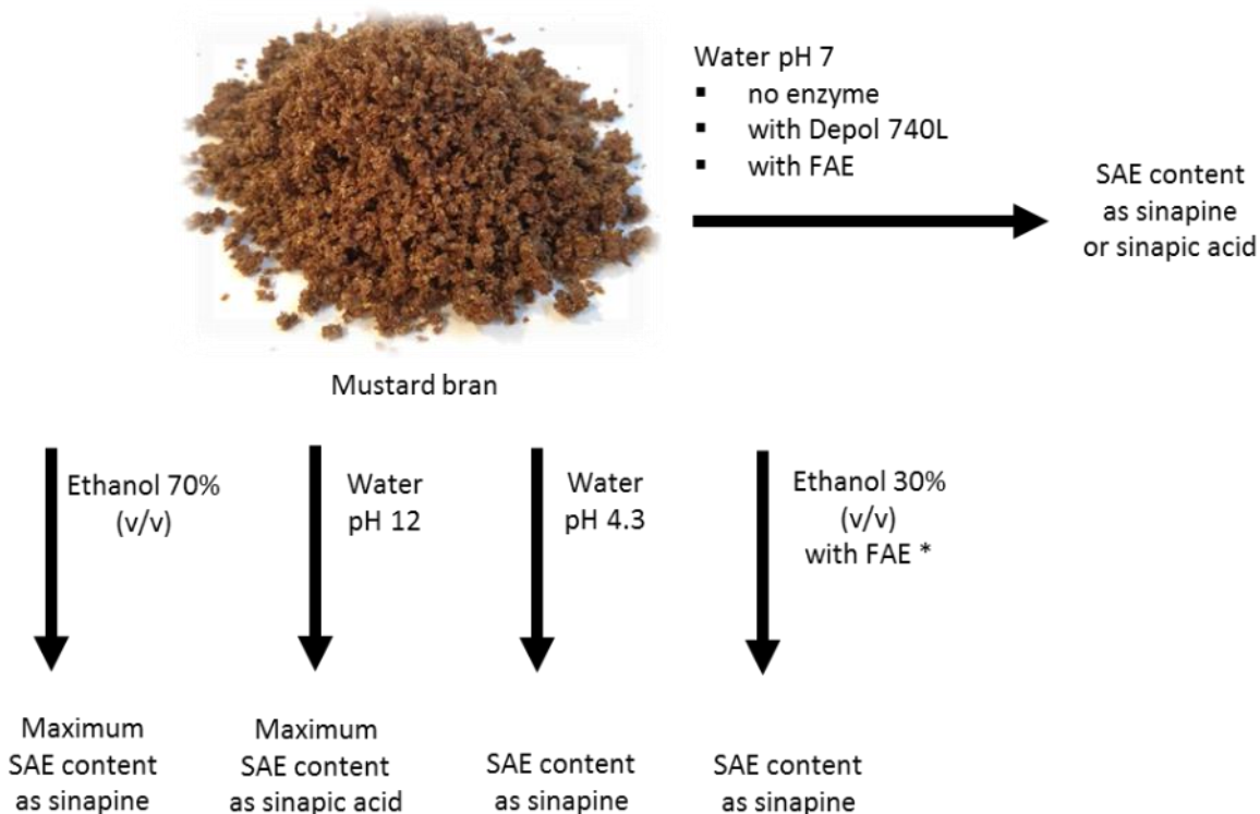
Figure 4: Flowchart of the different extractions on mustard bran. * Details in annex materials.
