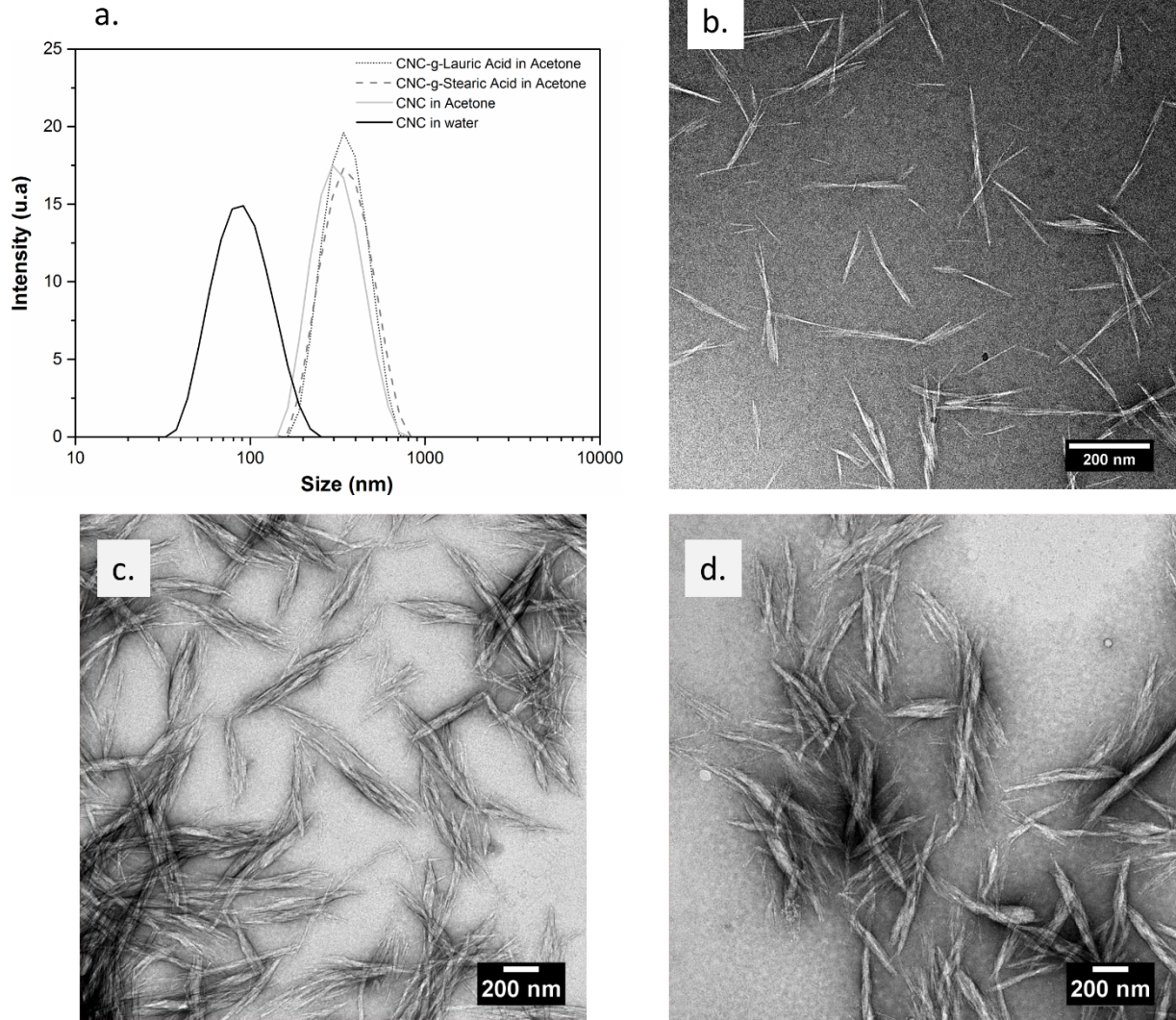
Figure 2. (a) DLS curves of unmodified CNC in water and acetone, and modified CNC in acetone. TEM images of (b) unmodified CNC in water, (c) CNC-g-lauric acid in acetone, and (d) CNC-g-stearic acid in acetone.
