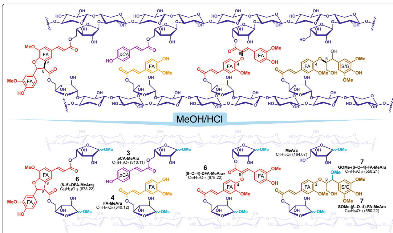
Fig. 1 Methanolysis of hydroxycinnamoylated arabinoxylan. Top: Schematic arabinoxylan chains shown with the arabinosyl substitutions on every second unit as revealed recently [39], along with p CA and FA substitutions on arabinosyl units, two representative diferulates (8-O-4 and 8-5) formed by radical coupling, and a monolignol ferulate (ML-FA) conjugate, all known to be present in grass cell walls; acetate substitutions, also known, are not shown. The bonds produced by radical coupling are shown in bold-black, and the bonds formed by post-coupling rearomatization reactions (along with the OH from water addition in the case of the ML-FA coupling) are in gray. Bottom: The derived products released for structural analysis and quantification upon methanolysis that, ideally, methanolizes the arabinosyl unit from the xylan backbone but leaves the arabinosyl esters intact. The original xylan chain is shown with low opacity for easier visualization of the source of the products, and the elemental formulas and exact mass (for MS analysis) are shown. As noted in the text, some actual hydrolysis can occur (producing acids) and some methanolysis of the hydroxycinnamate-arabinosyl ester can occur, producing DFAs with only a single Ara unit; the improved method here produces lower amounts of these undesirable side-products and more of the desired p CA-MeAra 3 , FA-MeAra 4 , and the various DFA-diMeAra isomers 6 (as well as ML-FA-MeAra cross-products 7 ); the compound numbers are from Fig. 2
