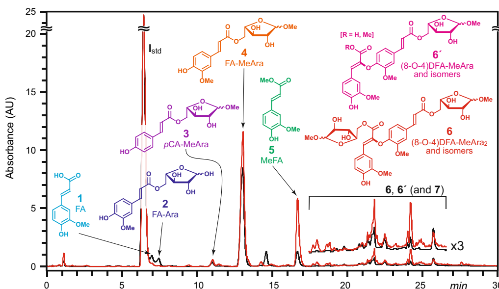
Fig. 2 UV-vis chromatograms of maize IDF after mild acidolysis. Black trace was processed using the original acidolysis method; red trace was the new anhydrous method described herein. Internal standard, I_{std} ; ferulate 1 ; FA-Ara 2 (unmethylated, m/z 325); p CA-MeAra 3 , FA-MeAra 4 ; MeFA, methyl ferulate, 5 ; DFAs 6 (one isomer, the 8- O -4-DFA, is shown) with two or one ( 6' ) MeAra attached, also shown vertically expanded \times 3 ; monolignol-FA-MeAra coupling products 7 (Fig. 1) are also in this region
