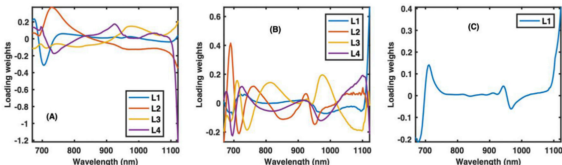
Fig. 6. Loading weights of the LVs extracted by SPORT for the olive data set. (A) MSC, (B) SNV, and (C) 2nd derivative.
