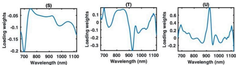
Fig. 7. Loading weights of the common and distinct components extracted by PORTO for the olive data set. Common component 1 (A–E), Common component 2 (F–I), Common component 3 (J–L), Common component 4 (M–O), Common component 5 (P–R), Distinct component corresponding to Raw (S), Distinct component corresponding to MSC (T), and Distinct component corresponding to VSN (U).
