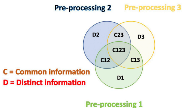
Fig. 2. A schematic illustration of the concept of common and distinctive information which constitutes the conceptual basis of PO-PLS and, as a consequence, of the PORTO approach to pre-processing fusion. The Fig. is adapted from the one presented in Ref. [19].
