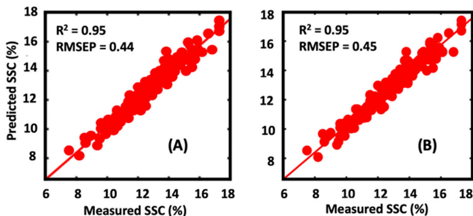
Fig. 8. PORTO model before and after pre-processing selection. (A) Preprocessings used: Raw+MSC+VSN+SNV+2nd derivative, and (B) Raw+MSC+2nd derivative.
