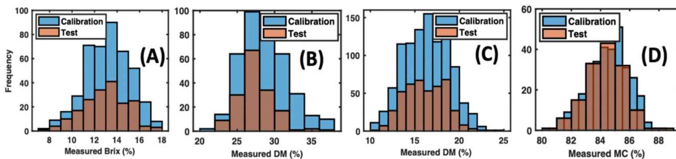
Fig. 3. Distribution of the reference values for each data set used for calibration and test set. (A) Apple data set, (B) Olive data set, (C) Mango data set, and (D) Pear data set.
