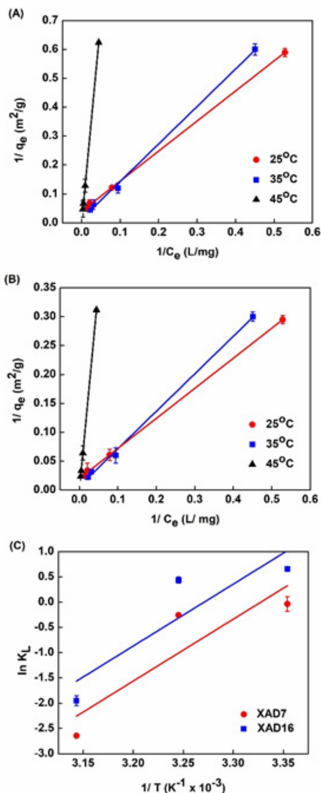
Figure 6: Equilibrium adsorption isotherm using the Langmuir model in linear form. (A) XAD7 and (B) XAD16 at 25°C, 35°C and 45°C; (C) \ln K_L vs. 1/T plot of adsorption equilibrium constant K_L using the Langmuir model.
