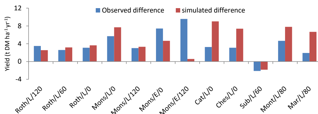
Figure 6. Histogram of differences between miscanthus and switchgrass annual yields, as observed (blue bars) or simulated by CERES-EGC (red bars) across the different experimental sites Rothamsted (Roth), Estrée-Mons (Mons), Catenoy (cat), Chesnoy (CHes), Subdray (Sub), Montant (Mont) and Marchais (Mar). For each region the difference is calculated for each cut (late (L) and early (E)), and each fertilization level (0, 60, 80 or 120 \text{kg N ha}^{-1} \text{yr}^{-1} ).
