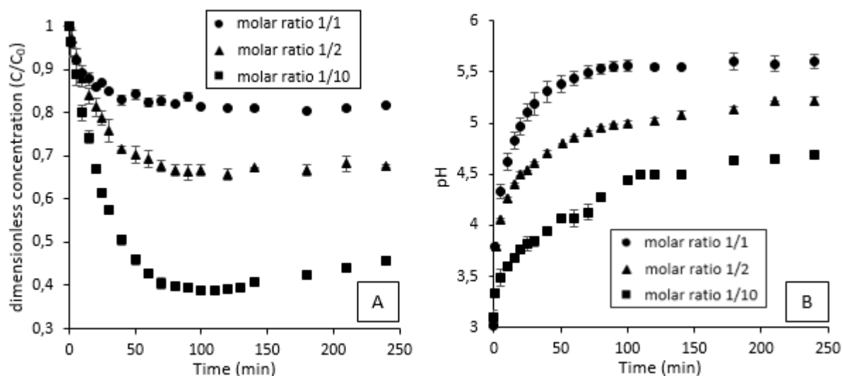
Figure 5. Dimensionless concentration of 3-HP (A) and pH evolution in the aqueous phase (B) over time for different initial \text{Cl}^- /3-HP molar ratios (initial concentration of 3-HP= 1 g/L).
