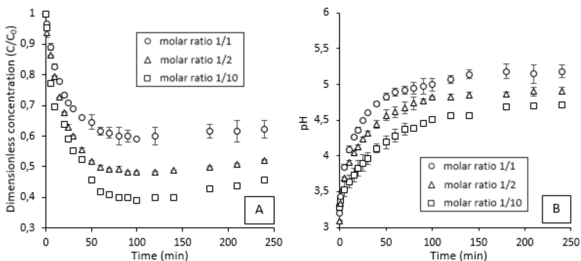
Figure 6. Dimensionless concentration of 3-HP (A) and pH evolution in the aqueous phase (B) over time for different initial \text{H}_2\text{PO}_4^- /3-HP molar ratios (initial concentration of 3-HP = 1 g/L).
