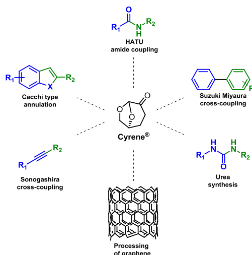
Scheme 2. The different applications of Cyrene® as green solvent
