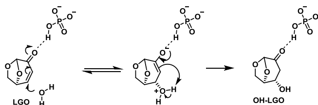
Scheme 4. Michael addition of water on LGO in phosphate buffer
