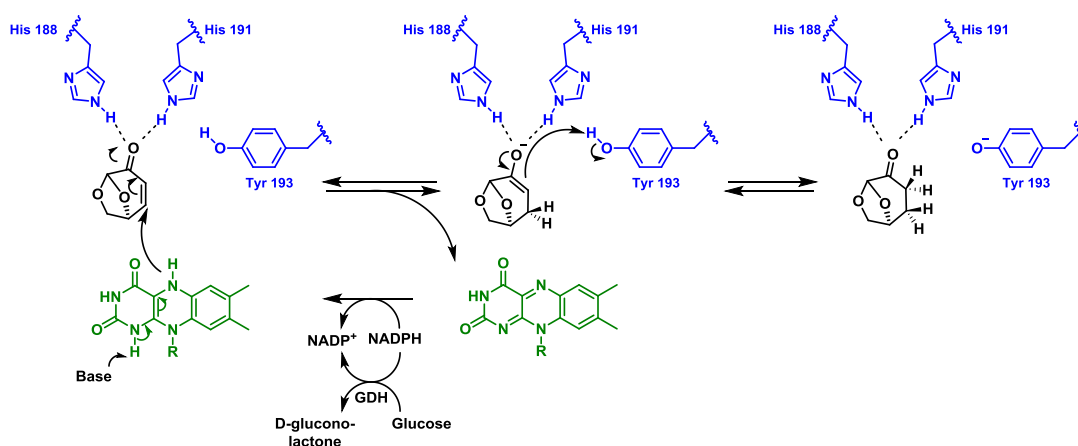
Scheme 3. Alkene reduction of Levoglucosenone into Cyrene ® using OYE 2.6 (Proposed mechanism)
