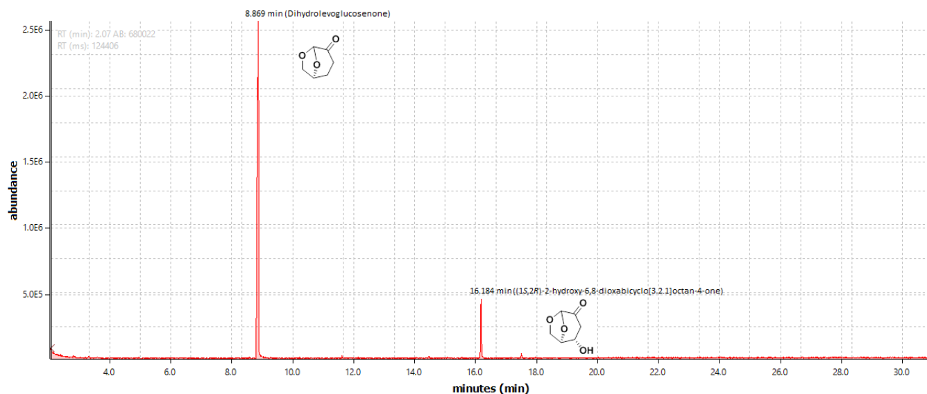
Figure 1. GC-FID analysis of non-optimized reaction conditions using OYE 26 Tyr 78 Trp
