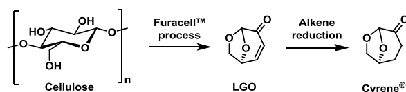
Scheme 1. Synthetic route to cellulose-based Cyrene®
