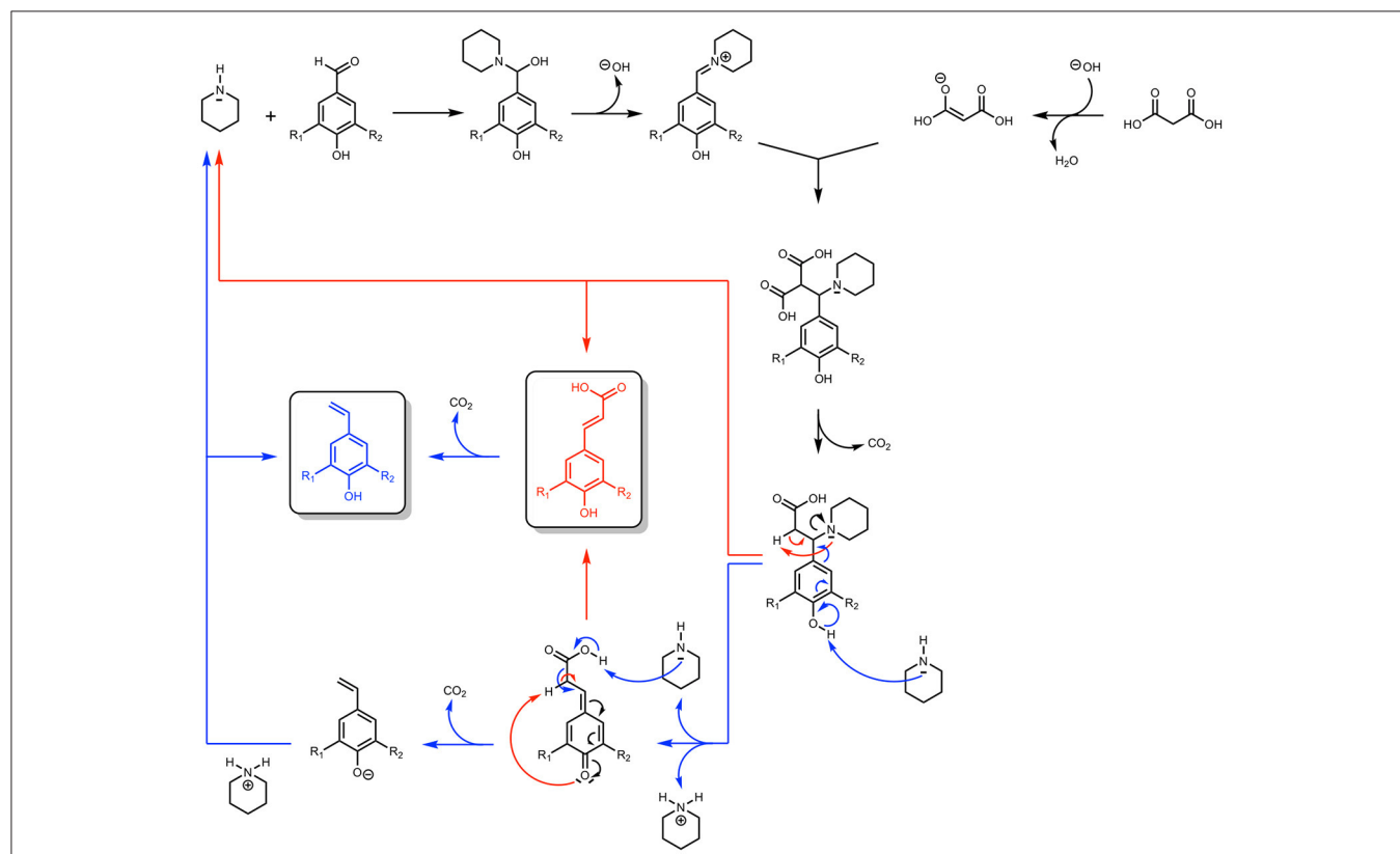
SCHEME 1 | Knoevenagel-Doebner condensation of p -hydroxybenzaldehydes using malonic acid and piperidine (Proposed mechanism).
