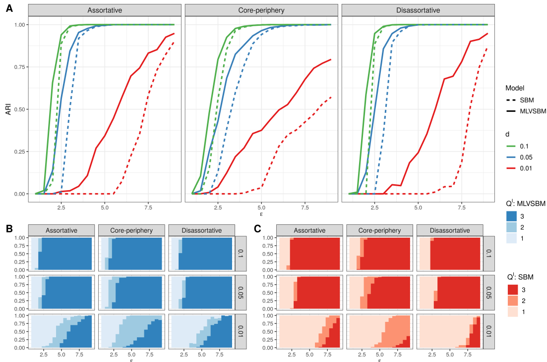
Figure 4: Clustering and model selection for 3 different topologies on the inter-individual level, varying \epsilon and density d . Each situation is simulated 50 times. A : ARI for the inter-individual level, comparing the model used for inference. B : Stacked frequency barplot of the selected number of blocks for the inter-individual level in the MLVSBM (in blue). C : Stacked frequency barplot of the selected number of blocks for the inter-individual level chosen in the SBM (in red).
