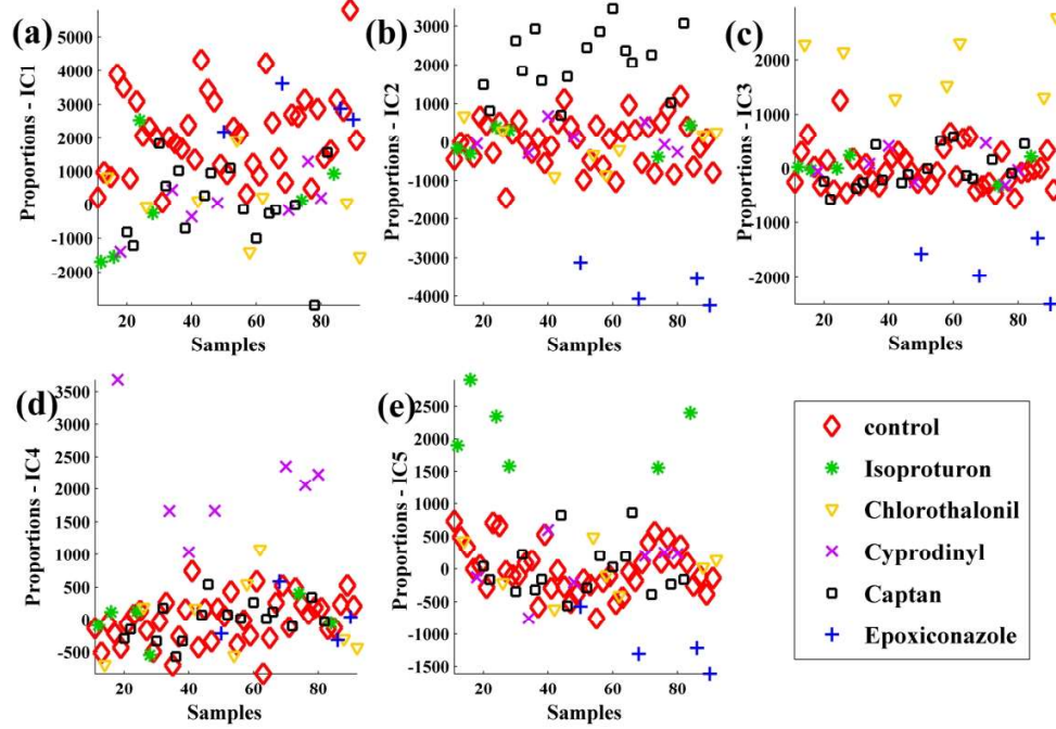
Fig. 1 Discrimination of control subjects (a) and exposure classes: captan (b), chlorothalonil (c), cyprodinyl (d), and isoprotruron (e). Results obtained from DIMS data processing without the contribution of group information, i.e., based only on the extracted MS source signals. Note that discrimination of epoxiconazole-exposed group is visible in another dimension (b, c and e).
