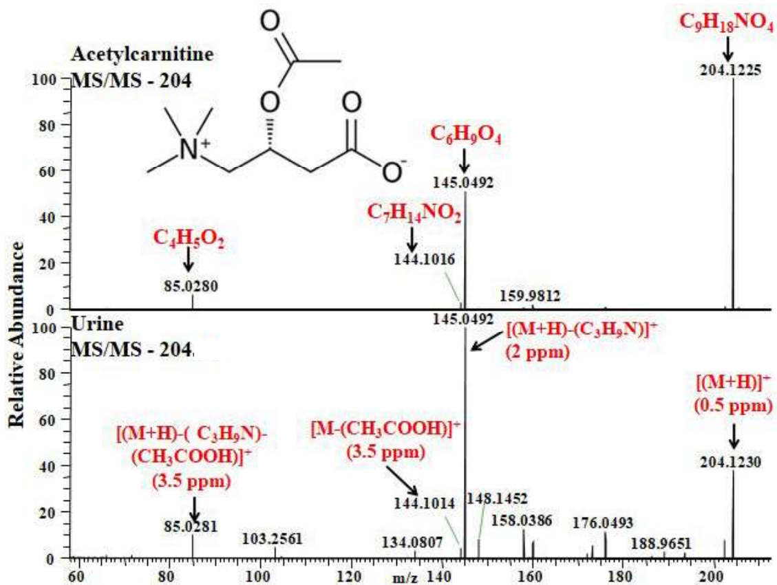
Fig.S.5 MS/MS spectra of the precursor [M + H]^+ ions at m/z 204 (a) from the authentic standard acetylcarnitine and (b) from a urine sample.
