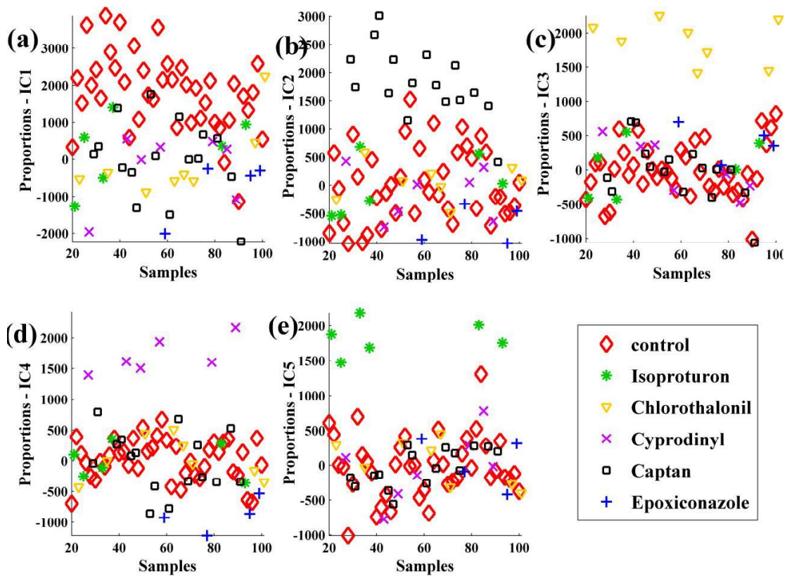
Fig.S.3 Results from LC/MS data processing without the contribution of group information, i.e., based on the only extracted MS source signals. A separation is still observed for captan, chlorothalonil, cyprodinyl and isoprotruron exposure groups ( b-e respectively). A discrimination of control subjects ( a ) is less apparent and no discrimination of epoxiconazol exposure group is obtained.
