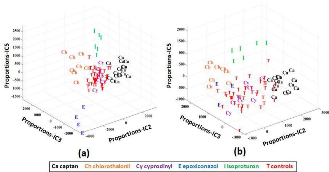
Fig.S.4 3D-plot from DIMS (a) and LC/MS (b) data processing without the contribution of group information. Discrimination of different exposure groups is observed, especially, separation of individuals exposed to isoproturon according to the proportions of IC-5. Cyprodinyl exposure group was discriminated according to another dimension as observed in Fig.2 .
