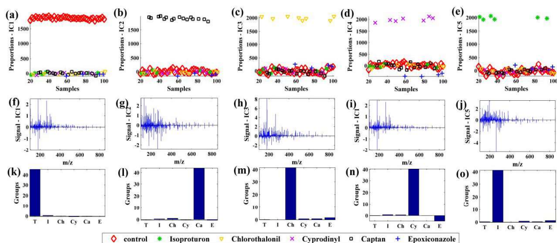
Fig.S.2 Results obtained from LC/MS data processing with known group memberships. Discrimination of control subjects (a) and all exposure classes: captan (b), chlorothalonil (c), cyprodinyl and epoxiconazol (d) and isoprotruron (e). The corresponding extracted source signals show the m/z values which most contribute to group discrimination (f, g, h, i and j plots). The peak intensity represents the ion contribution to the corresponding IC. The part of the source signals belonging to the group membership matrix show which group(s) contribute(s) the most to build the IC when compared to the influence of the others (k, l, m, n and o).
