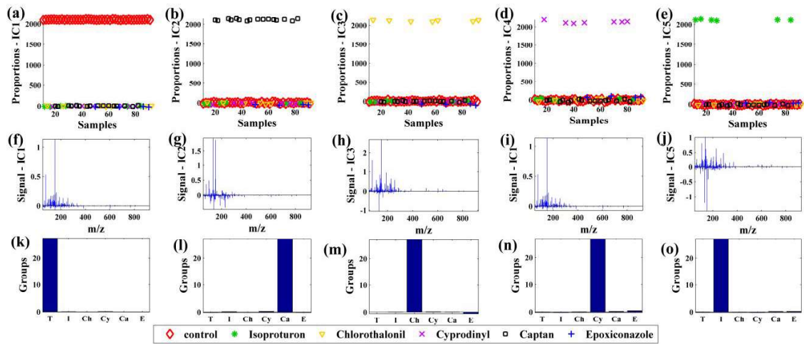
Fig.S.1 Results obtained from the DIMS data processing with known group memberships. Discrimination of control subjects (a) and the four exposure classes: captan (b), chlorothalonil (c), cyprodinyl (d) and isoproturon (e). The corresponding extracted source signals show the m/z values which most contribute to group discrimination (f, g, h, i and j). The peak intensity represents the ion contribution to the corresponding IC. The part of the source signals belonging to the group membership matrix show which group(s) contribute(s) the most to build the IC when compared to the influence of the others (k, l, m, n and o). Note that no discrimination is observed for epoxiconazole-exposed subjects.
