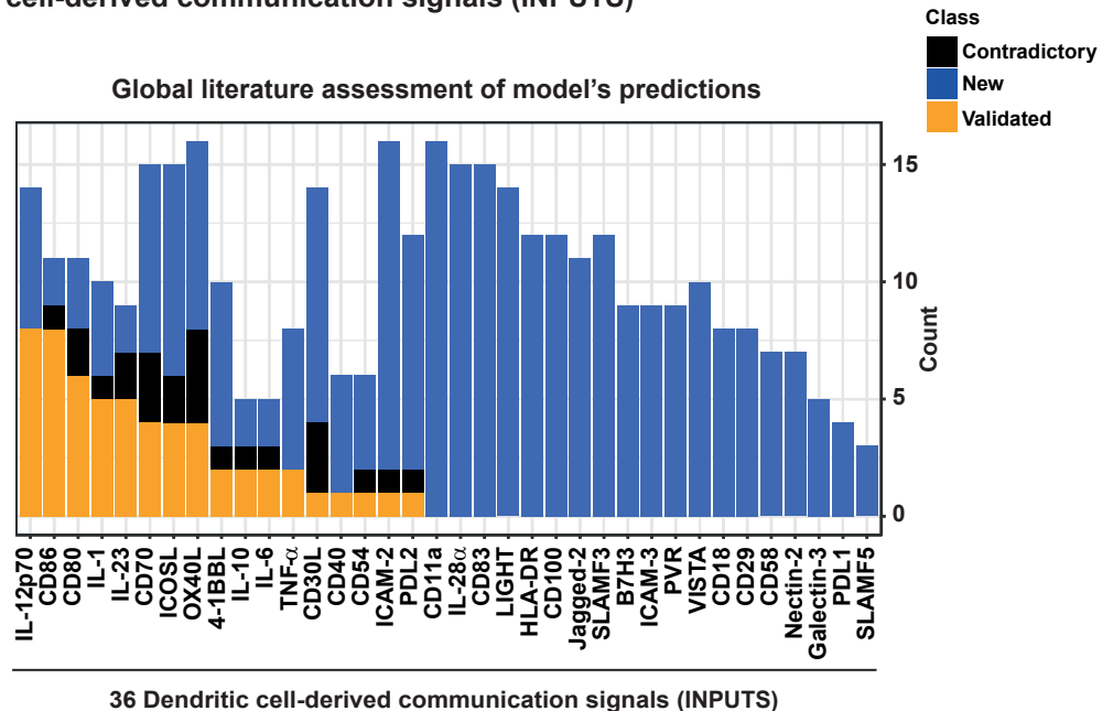
FIGURE 4: A data-driven Lasso penalized regression model predicts multiple Th differentiation outcomes from DC-derived communication signals expression
