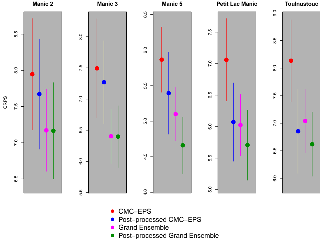
Figure 15: CRPS (in mm) for 2014 post-processed 9-days ensemble cumulative precipitation forecasts and associated bootstrap intervals. Year 2013 is used to estimate the parameters.
