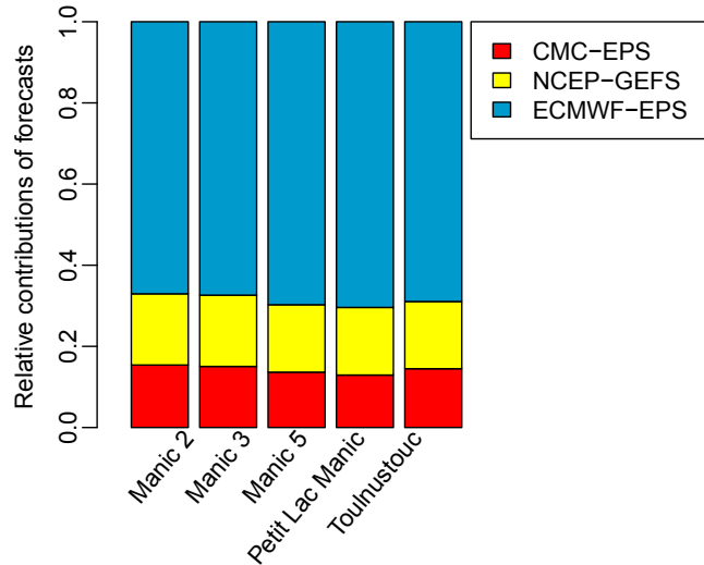
Figure 12: Relative contributions of forecast sources according to the two-variable latent model averaged over the nine forecast lead times.
