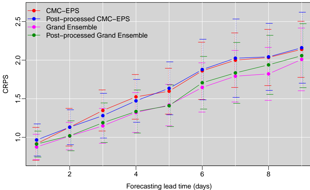
Figure 14: CRPS (in mm) for 2014 post-processed ensemble precipitation forecasts for the Manic 2 watershed as a function of the lead times and with associated bootstrap intervals. Year 2013 is used to estimate the parameters.
