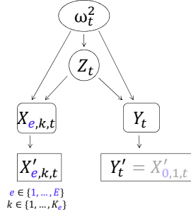
Figure 3: Direct acyclic graph of the post-processing model for precipitation. X'_{e,k,t} denotes the k^{th} member of ensemble e at time t , K_e is the size of the ensemble e , Y'_t = X'_{0,K_0=1,t} = X'_{0,t} denotes the variable to forecast and \mathbf{X}_t , Y_t , Z_t and \omega_t^2 are latent variables (partially observed in the case of \mathbf{X}_t and Y_t ). Times are assumed to be independent.
