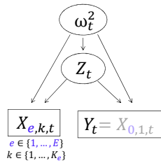
Figure 2: Directed acyclic graph of the model given by Eq 4. X_{e,k,t} is the k^{th} member of the ensemble e at time t and K_e is the number of members from the ensemble e , Y_t = X_{0,K_0=1,t} = X_{0,t} relates to the targeted variable to forecast, and Z_t and \omega_t^2 are the model backbone latent variables. Times are assumed to be independent.
