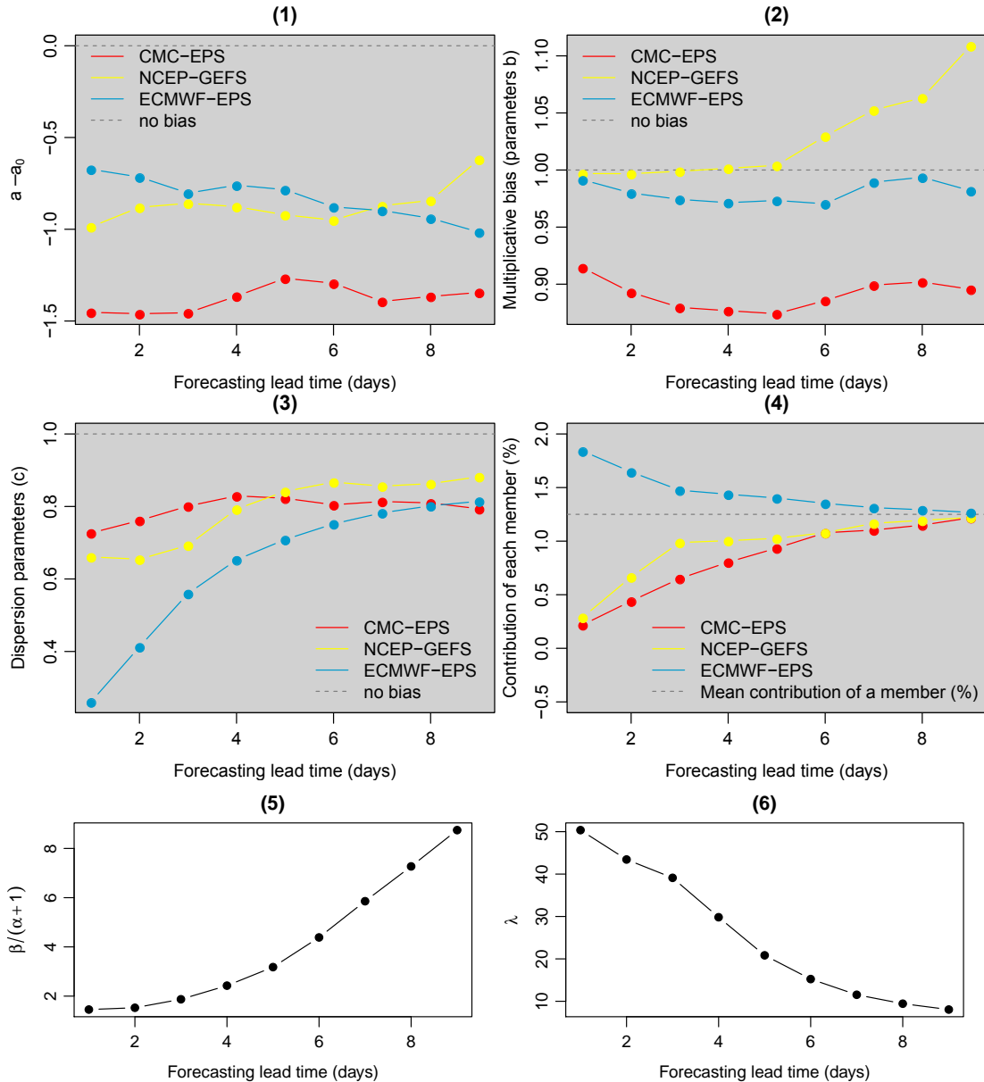
Figure 8: Parameters obtained with the EM algorithm are represented as a function of the forecasting horizon for the Manic 2 watershed with E = 3 forecasting sources (CMC-EPS, NCEP-GEFS and ECMWF-EPS). Year 2013 has been used as the learning period.
