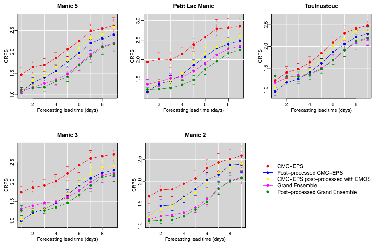
Figure 11: CRPS (in ^{\circ}\text{C} ) for maximum temperature forecasts for the five catchments for all 9 lead times with associated bootstrap intervals. The parameters have been estimated using year 2013 and verification has been performed for year 2014.
