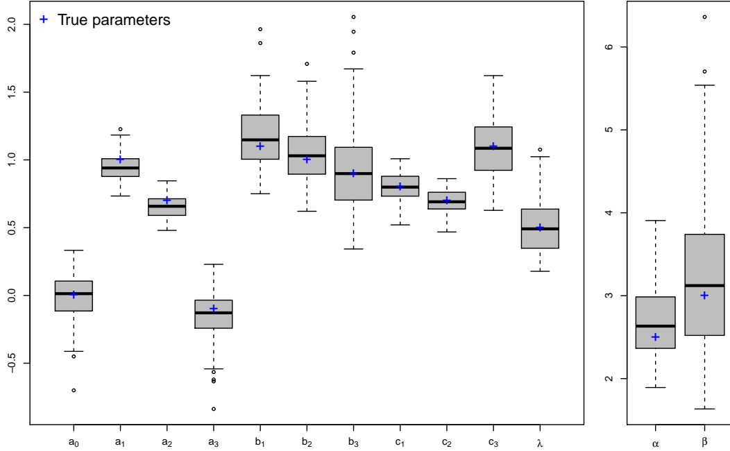
Figure 4: Parameters obtained after inference from 100 simulations of 100 repetitions according to the precipitation model. The parameters used for the simulation are represented by the blue crosses.
