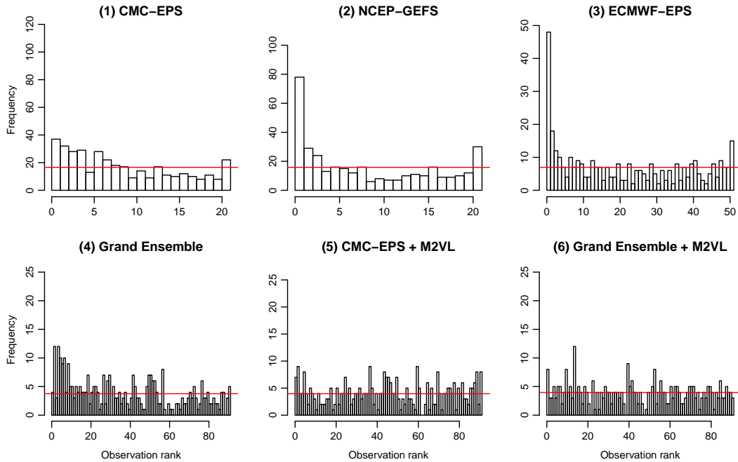
Figure 1: Rank histograms for 3-days lead time ensemble precipitation forecasts produced daily in 2014 for Manic 2 watershed: (1) CMC-EPS raw ensemble (2) NCEP-GEFS raw ensemble (3) ECMWF-EPS raw ensemble (4) large raw ensemble gathering CMC-EPS, NCEP-GEFS and ECMWF-EPS members (5) post-processed CMC-EPS (6) post-processed large ensemble.
