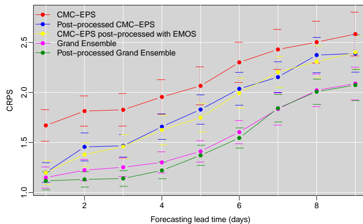
Figure 10: CRPS (in ^{\circ}\text{C} ) for maximum temperature forecasts at Manic-2 catchment for all 9 lead times with associated bootstrap intervals. The parameters have been estimated using year 2013 and verification has been performed for year 2014.
