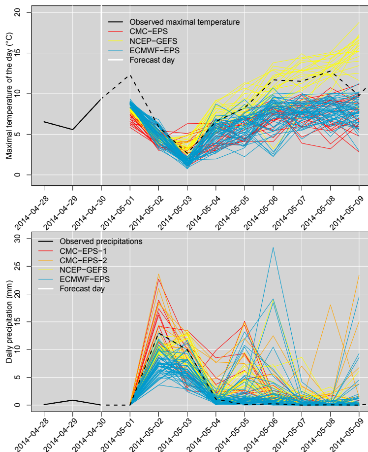
Figure 7: Precipitations and maximal temperature raw ensemble forecasts on the Manic 2 watershed produced the 30 of April 2014 for the nine upcoming days (CMC-EPS, odd members: 1 and even members: 2, NCEP-GEFS and ECMWF-EPS). The target values, to be predicted, are indicated by the dotted black line.
