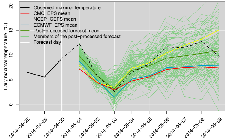
Figure 9: Example of a forecast issued for the daily maximum temperatures of the Manic 2 catchment area with the proposed post-processing method taking NCEP-GEFS, CMC-EPS and ECMWF-EPS as inputs. Predictive scenarios derived from meteorological forecasts by forecast time horizon using the ECC-Q are presented. The maximum daily temperature to be forecast (observed afterward) is indicated by the black dotted line.
