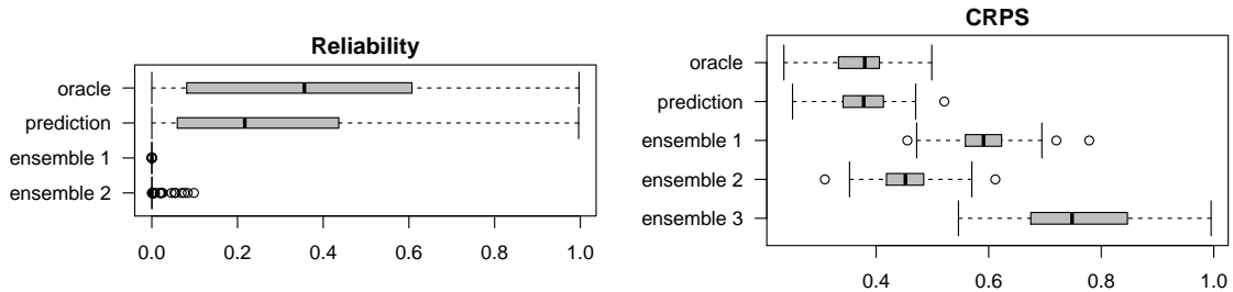
Figure 5: Reliability (left-hand-side) and CRPS (right-hand-side) of forecasts issued by post-processing approaches computed over 100 datasets simulated according to the precipitation model. Reliability is here summarized by the p-values of the multinomial goodness-of-fit Chi-squared tests which compare the rank histograms to a flat histogram. oracle and prediction refer to our post-processing method with respectively true and estimated parameters. They are compared with the three raw ensembles considered as probabilistic forecasts (Reliability of Ensemble 3 is omitted since it is a single member ensemble).
