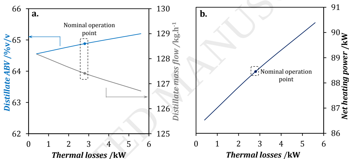
Fig. 15. Influence of heat losses on a. distillate ethanol composition and mass flow and b. heat power. In this simulation, the ethanol losses in the bottoms as well as the condensation power were fixed at the nominal point values. 2-column fitting image.
