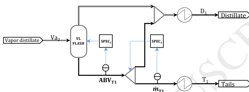
Fig. 10. Configuration for the simulation of a. heads and b. tails extractions. SPEC_1 and SPEC_2 are control loops to verify the respective experimental values of ethanol composition ( ABV ) and mass flow ( \dot{m} ) of the extraction. 1.5-column fitting image.
