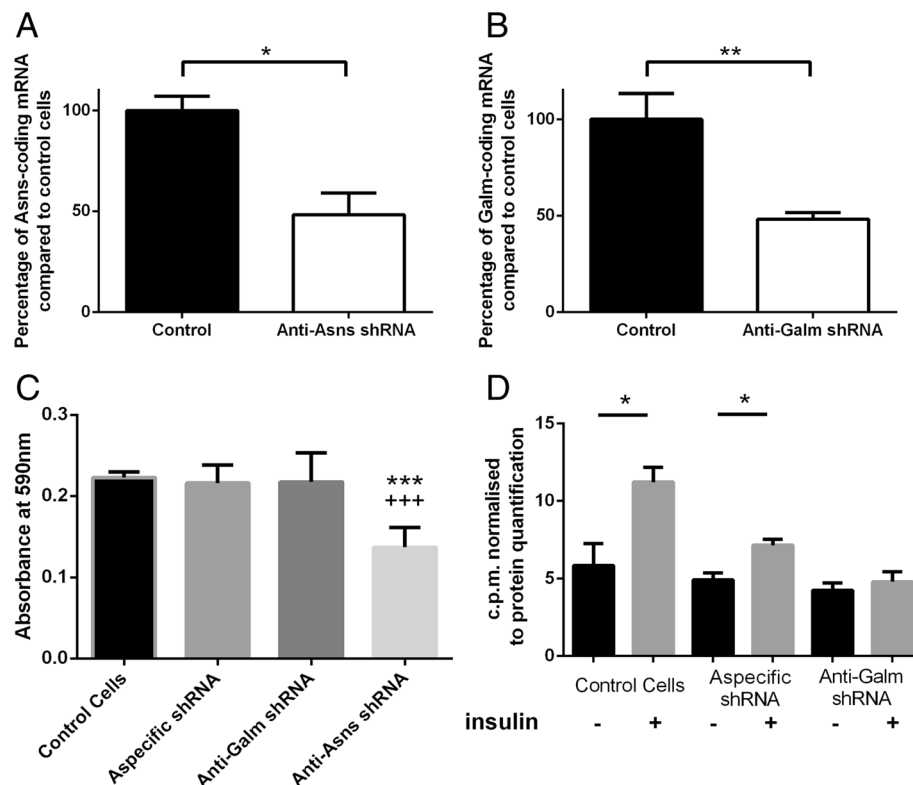
Fig. 5 Functional assessment of in vitro shRNA-mediated inhibition of Galm and Asns expression in 3T3-L1 adipocytes. a Asns mRNA expression levels in anti- Asns shRNA-treated cells expressed as a percentage of control 3T3-L1 cells. b Galm mRNA expression levels in anti- Galm shRNA-treated cells expressed as a percentage of control 3T3-L1 cells. c Intracellular lipid content of differentiated 3T3-L1 cells was measured by absorbance at 590 nm after Oil Red-O staining. d Glucose uptake was evaluated by measurement of radiolabeled 2-deoxyglucose present in 3T3-L1 cells following insulin stimulation and normalized to protein level. Shown data represent means \pm standard error of the mean. Mann-Whitney tests were performed: * P < 0.05 , ** P < 0.01 , and *** P < 0.001 significantly different to control; and +++ P < 0.001 significantly different to Galm -deficient cells
