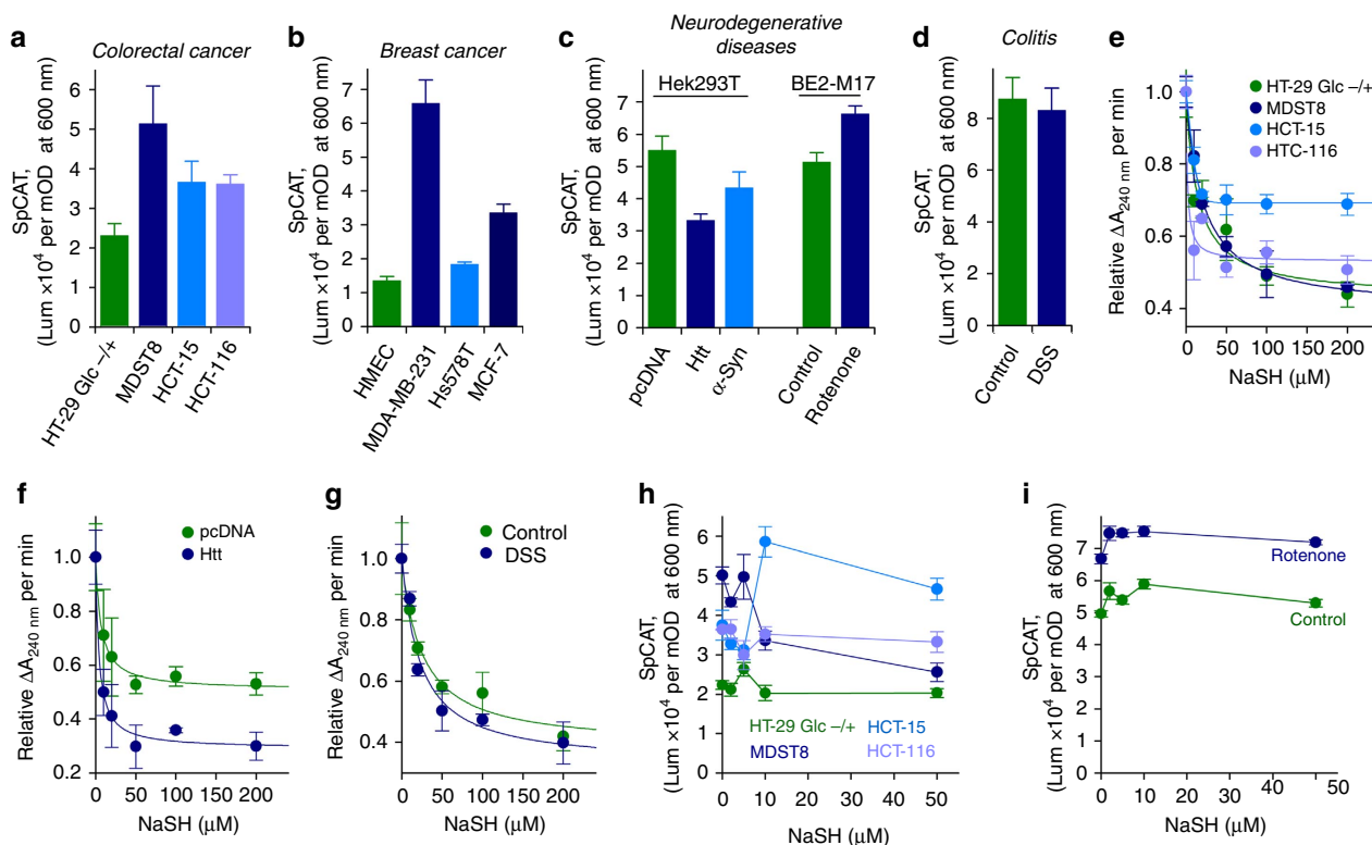
Figure 6 | HCys-induced sulcatase formation is likely in various pathological disorders. (a) Relative specific activity of immunocaptured catalase (SpCAT) in various human colorectal cancer cells. The HT-29 Glc -/+ cell line was chosen as a control as it maintains metabolic characteristics of normal colonocytes. (b) Comparison of SpCAT in human mammary epithelial cells (HMEC-control) and in various HBC cells. (c) SpCAT measured in diverse cellular models of neurodegenerative disorders: Hek 293T cells transfected with an empty plasmid (pcDNA-control), Htt-N171-82Q (Htt) or Alpha-synuclein-A53T (α-Syn) and M17 human neuroblastoma cells treated or not (control) with 100 nM rotenone. (d) SpCAT in crypt and surface epithelial cells isolated from a rodent model of DSS-induced colitis (DSS) in comparison with untreated mice (control). (e–g) Dependency of H 2 O 2 consumption in various cell lysates on the concentration of NaSH. Cell lysates were preincubated with NaSH on ice for 5–10 min before monitoring H 2 O 2 disappearance at 240 nm. (h,i) Dependency of SpCAT on the concentration of NaSH in various human colorectal cancer cells (h) and in a cellular model of Parkinson's disease (i). Data are represented as means ± s.d. (colorectal cancer cells and neurodegenerative diseases, n = 2; breast cancer cells and colitis, n = 3). Each experiment was performed in duplicate (SpCAT) or triplicate (H 2 O 2 consumption).
