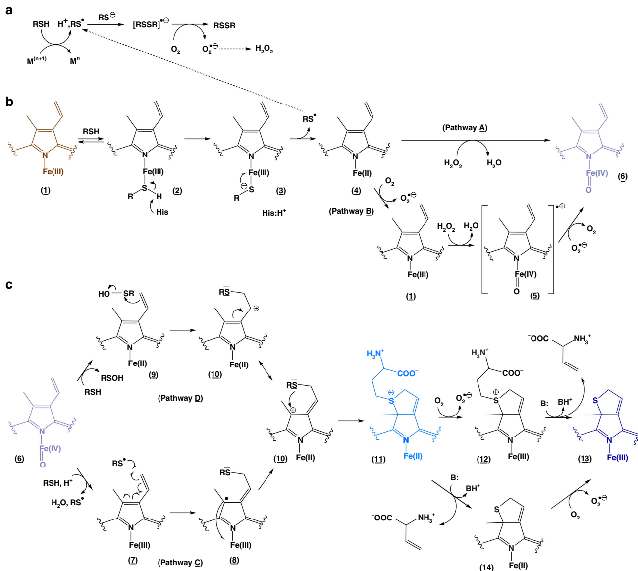
Figure 3 | Possible reaction routes for HCys-induced sulfheme formation. (a) In the presence of copper or iron, RSH can enter into a futile redox cycling to generate thiyl radicals ( \text{RS}^\bullet ), superoxide anion radicals ( \text{O}_2^{\bullet\ominus} ) and \text{H}_2\text{O}_2 which originates from the dismutation of the latter. (b) Possible mechanisms for the formation of compound II from CAT-Fe(III) in the presence of RSH. (c) Possible mechanisms for the generation of sulfheme from compound II in the presence of RSH. In here RSH represents HCys.
