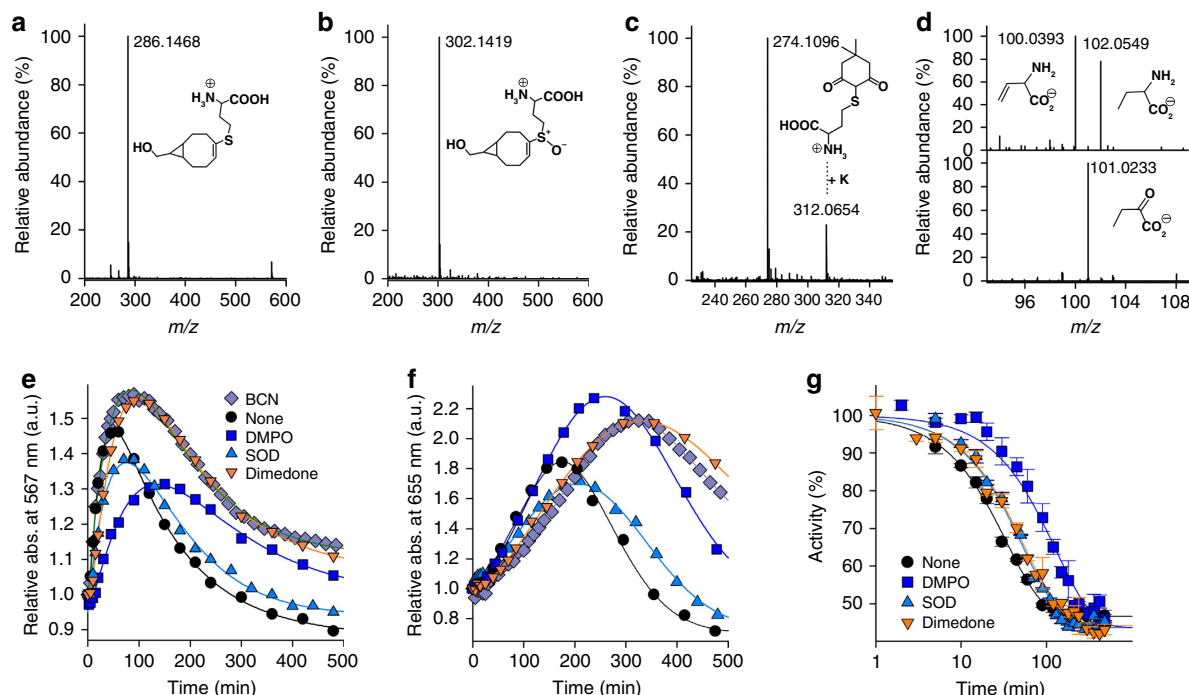
Figure 4 | Thiyl radicals and sulfenic acid species intervene during sulfheme formation. (a–d) High-resolution mass spectra of the BCN (a,b) and dimedone (c) adducts ( \text{ESI}^+ ) as well as the HCys derivatives (d; \text{ESI}^- ) formed during the reactivity of catalase ( 3\mu\text{M} ) with HCys ( 2\text{mM} ). (e,f) Comparative kinetic studies of \text{CAT-Fe(IV)=O} formation (e) and \text{CAT-Fe(II)} sulfonium generation (f) when catalase ( 1.75\mu\text{M} ) is exposed to 2\text{mM} HCys in the absence or the presence of various additives. (g) Time course of catalase inactivation observed under the same experimental conditions as those described in (e,f). The k_{\text{inact}} values extracted from the analysis of the plots are reported in Table 2 ( n=2\pm\text{s.d.} ).
