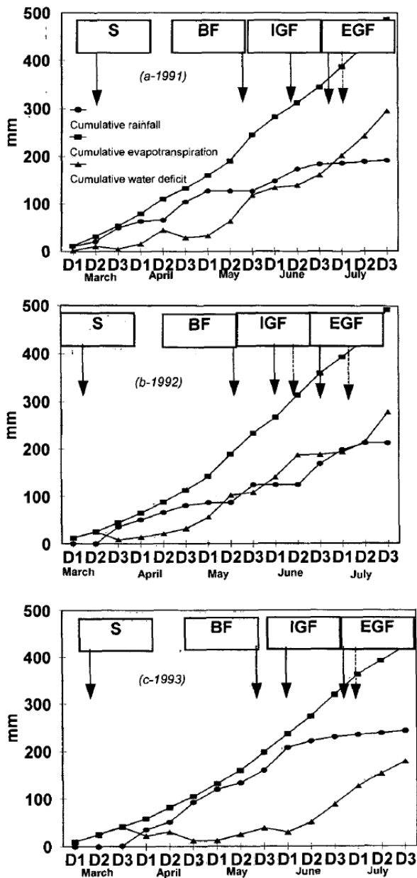
Fig. 1. The climate during the three years of a field irrigation timing experiment (1991 = a; 1992 = b; 1993 = c) on ‘ Solara ’ pea. S = sowing date, BF = beginning of flowering, IGF = initiation of seed filling (----- for WI treatment and — for NI treatment), EGF = end of seed filling (----- for WI treatment and — for NI treatment). D1, D2 and D3 are the first, second and third decade of each month, respectively.
