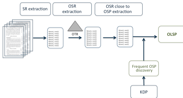
Figure 4: The hybrid approach of Xart system
