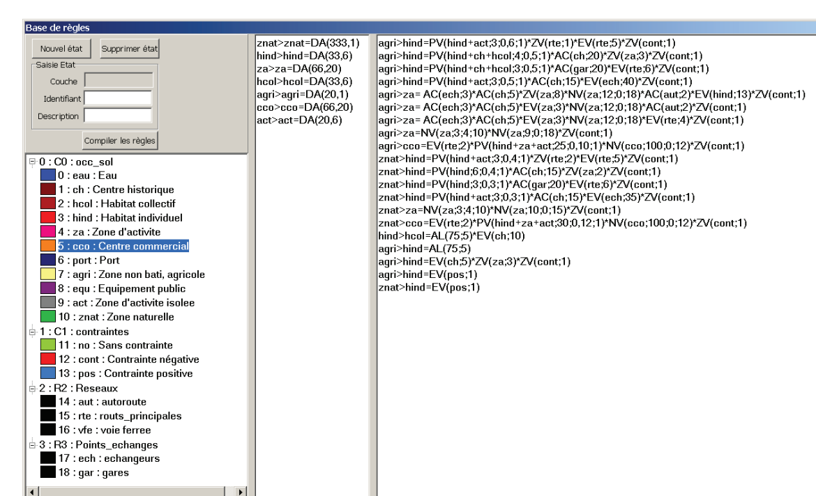
Fig. 3: 'Spacelle' cellular automata interface (v. 5.1.8): Definition of states and rules. Application of Montpellier case study. Spacelle is developed by P. Langlois, University of Rouen
