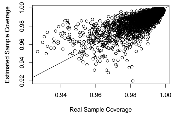
(b) Geometric distribution. The estimated sample coverage is 1.046 times the real one minus 0.046, with an R^2 value around 69%.
