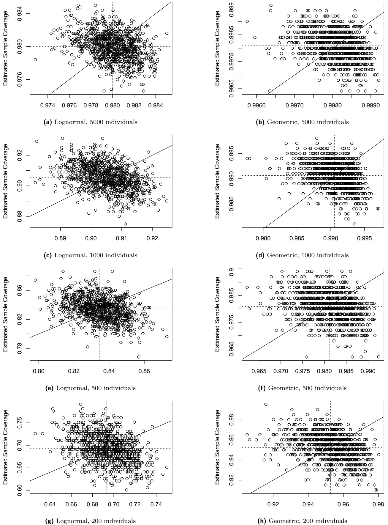
Figure 8. Estimated vs real sample coverage of simulated samples. The dotted lines are the average values. The distributions contain 600 species. The plain line represents equality.
