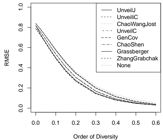
(b) Geometric distribution
