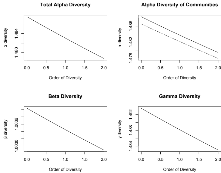
Figure 2: Functional diversity profile of the Paracou forest communities. Top left: \alpha diversity of the meta-community; top right: \alpha diversity of each community (P006: plain line, P018: dotted line); bottom left: \beta diversity; bottom right: \gamma diversity. Diversity is the number of effective species (effective communities for diversity) against the order q . It is estimated with bias correction.
